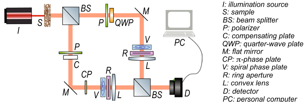
Fig. 7 Mach-Zehnder interferometer for orbitalization ellipsometry measurements
