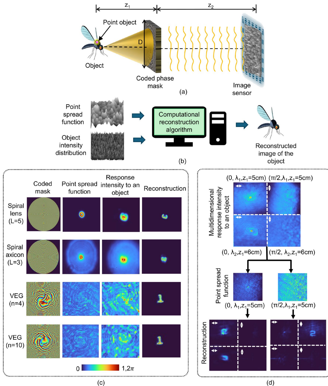
Fig. 15 Optical configuration of I COACH a Recording and b reconstruction process. Experimental results c CMs, PSFs, RIOs, and reconstruction results by LRRAs of the spiral lens ( L = 5 ), spiral axicon ( L = 3 ), VEG ( n = 4 ), and VEG ( n = 10 ). The variables L and n indicate the topological charge and number of spiral phase elements, respectively.
